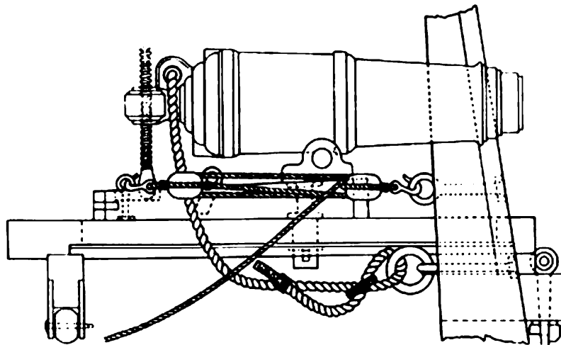
24 PDR. CARRONADE
